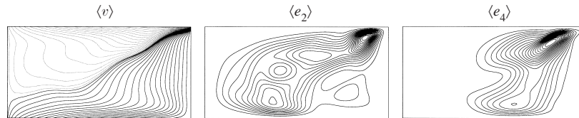
FIGURE 28. Contours of the azimuthally averaged azimuthal velocity and azimuthally averaged modal energy density for MRW_{2,0} at S = 0.800 ; \max(e_2) = 4.5 \times 10^{-3} , \max(e_4) = 1.1 \times 10^{-2} .
